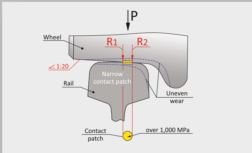
Conventional railway wheel
