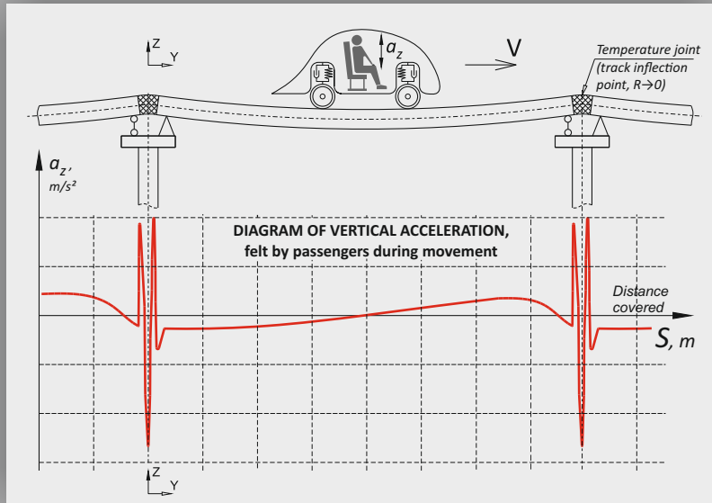
SPLIT OVERPASS (CONVENTIONAL BRIDGE)
