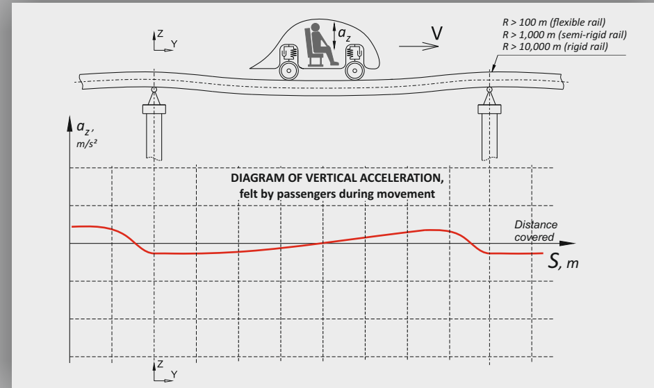
UNCUT PRE-STRESSED OVERPASS (SkyWay TECHNOLOGY)
